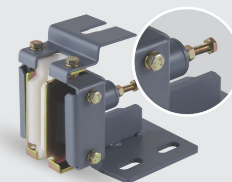
Guide Shoe ECGS-04ST
