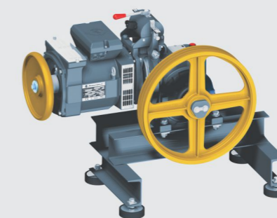
M 67 Traction Machine
